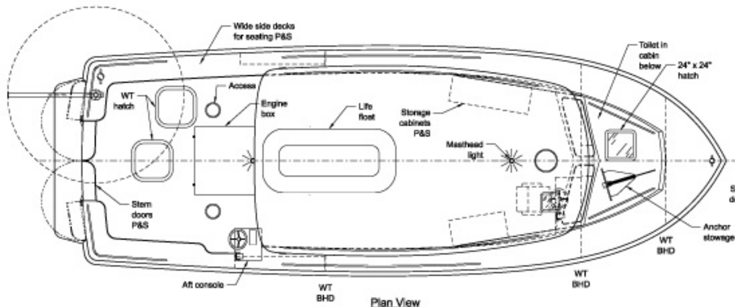
Plan View
