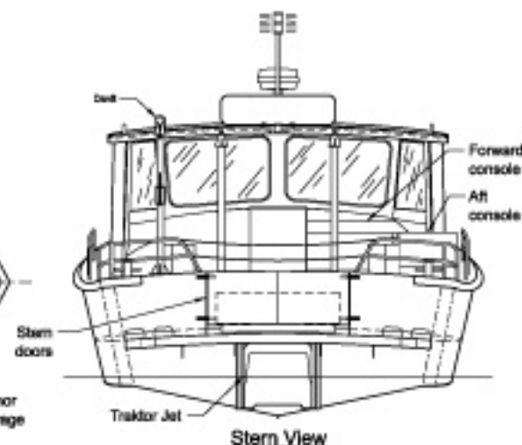
Stern View
