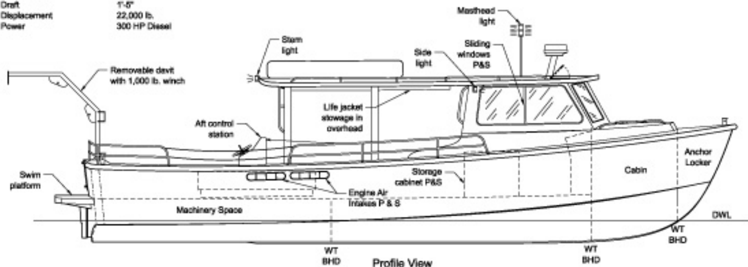
Profile View
